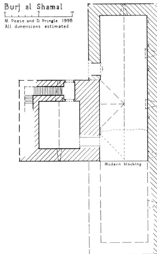
Fig. 7 – Burj al-Shamālī: sketch plan of the tower and vault (© drawn by Matthew Pease).
