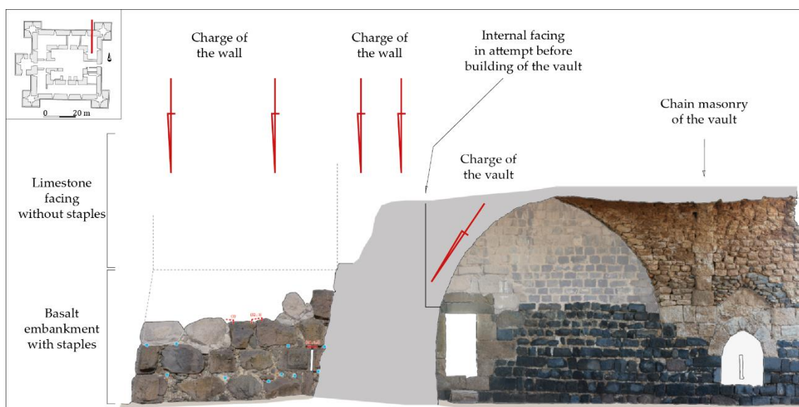
Fig. 4 – Construction method of the central building of the castle of Belvoir (© L. D'Agostino).
